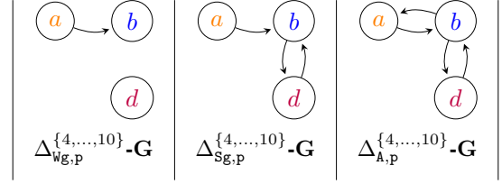
Figure 2: \mathbf{G} between 4 and 10 according to a \Delta
